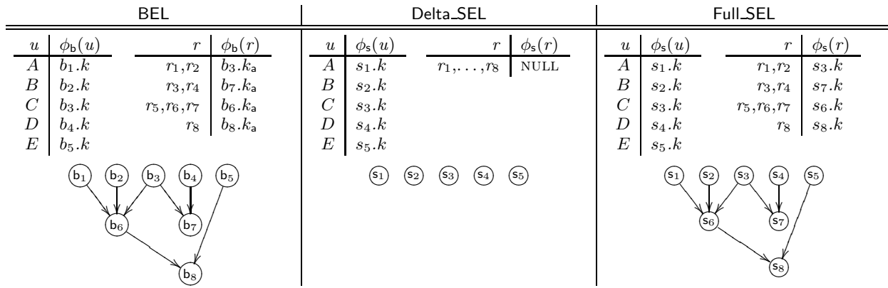
Figure 4: An example of BEL and SEL combination with the Delta_SEL and the Full_SEL approaches
