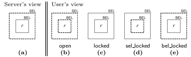
Figure 7: Possible views on resource r
